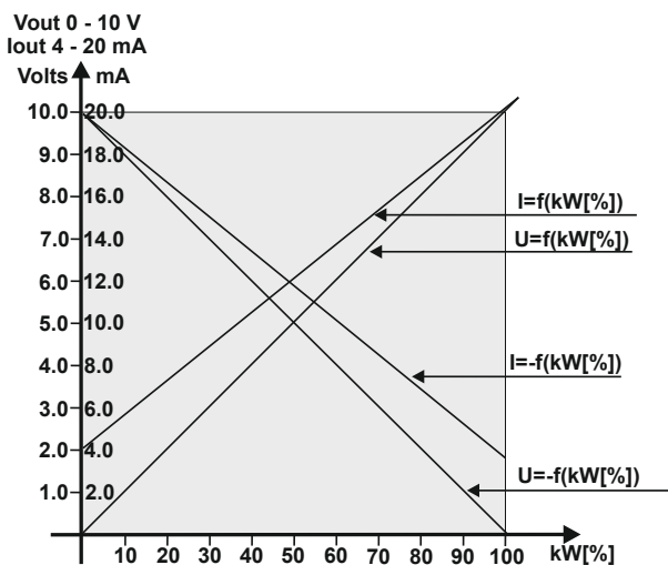
Analog Output 0 - 10Volt and 4-20mA Normal and Inverted
